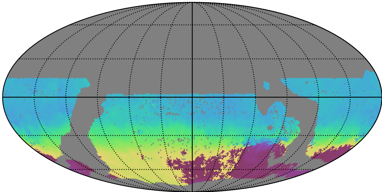
mw_roll_all_v3.3_10yrs WFD r band: AngleMean rotSkyPos
