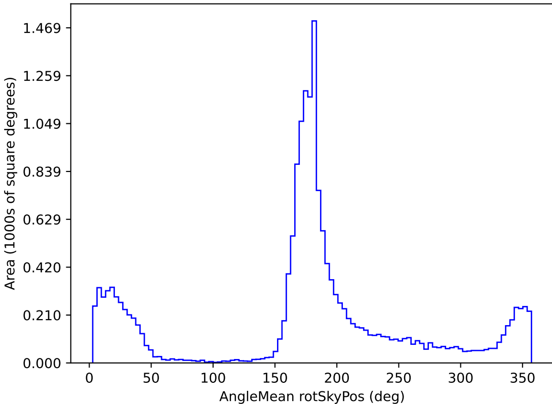
mw_roll_all_v3.3_10yrs WFD g band: AngleMean rotSkyPos
