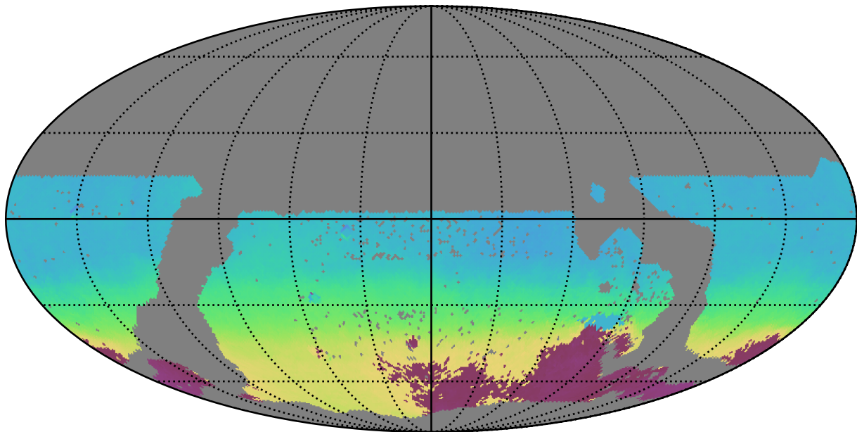
mw_roll_all_v3.3_10yrs WFD all bands: AngleMean rotSkyPos
