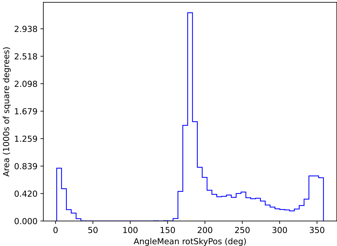
mw_roll_all_v3.3_10yrs WFD all bands: AngleMean rotSkyPos
