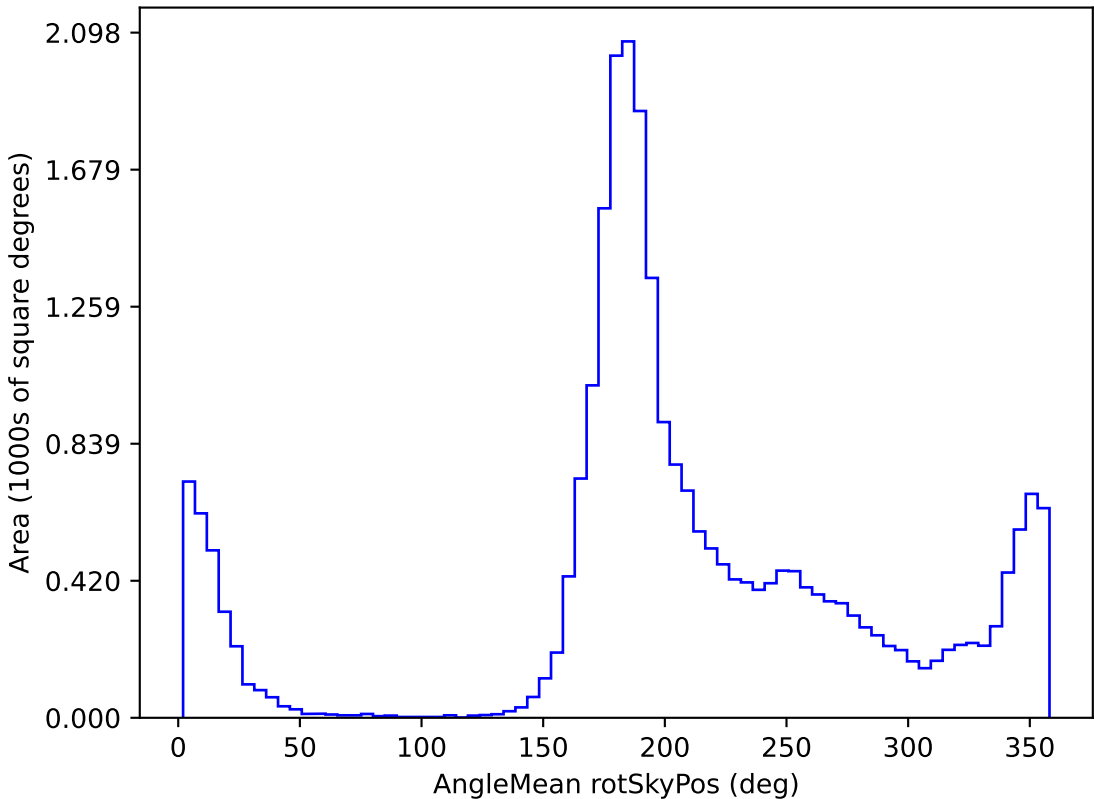
mw_roll_all_v3.3_10yrs All sky z band: AngleMean rotSkyPos
