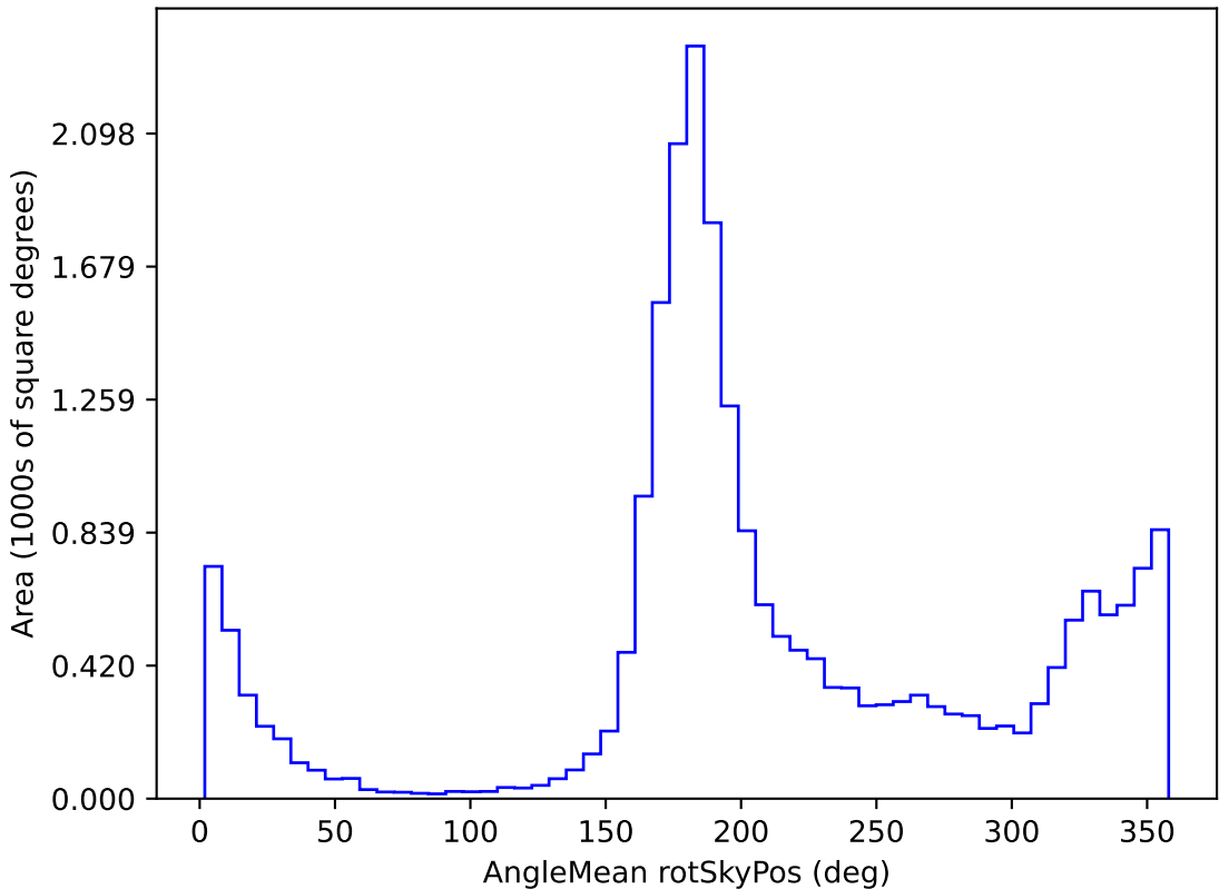
mw_roll_all_v3.3_10yrs All sky u band: AngleMean rotSkyPos
