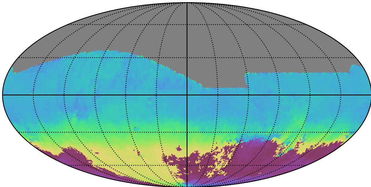
mw_roll_all_v3.3_10yrs All sky r band: AngleMean rotSkyPos
