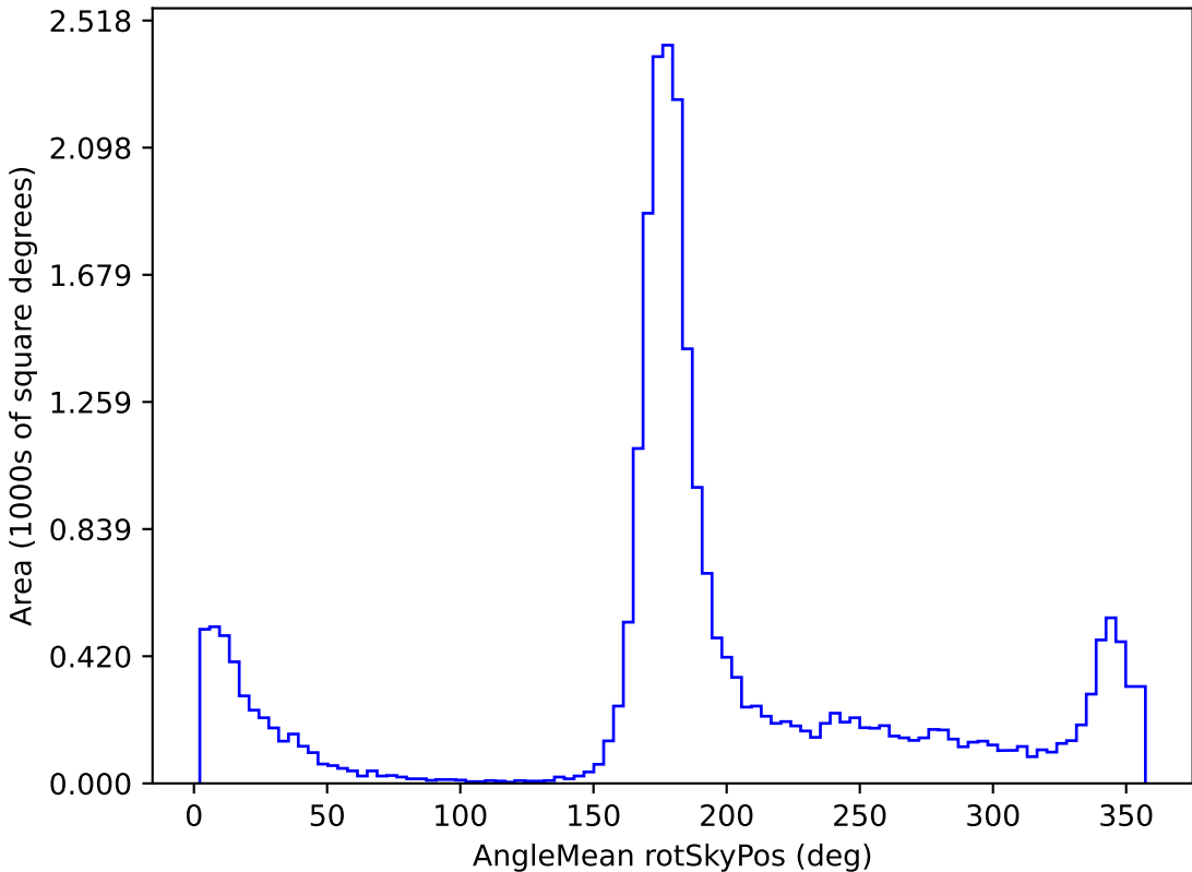
mw_roll_all_v3.3_10yrs All sky r band: AngleMean rotSkyPos
