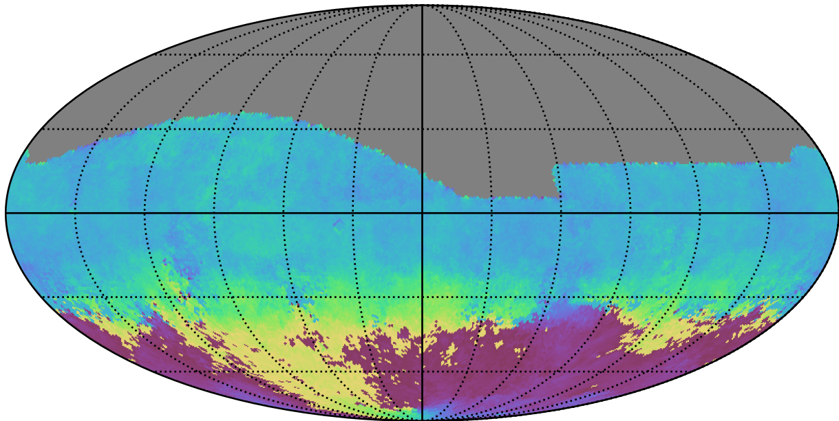
mw_roll_all_v3.3_10yrs All sky g band: AngleMean rotSkyPos
