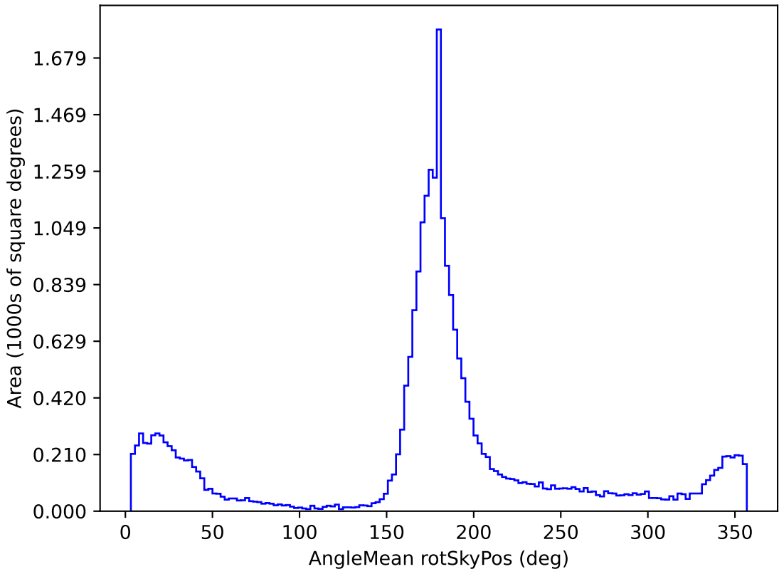
mw_roll_all_v3.3_10yrs All sky g band: AngleMean rotSkyPos
