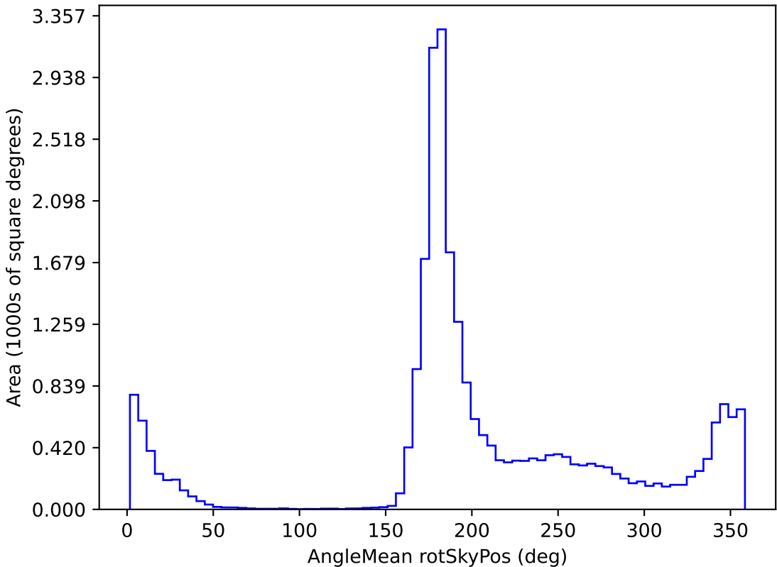
mw_roll_all_v3.3_10yrs All sky all bands: AngleMean rotSkyPos
