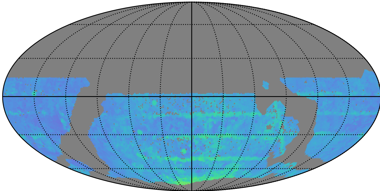
mw_roll_all_v3.3_10yrs WFD z band: 80thPercentile Season Length
