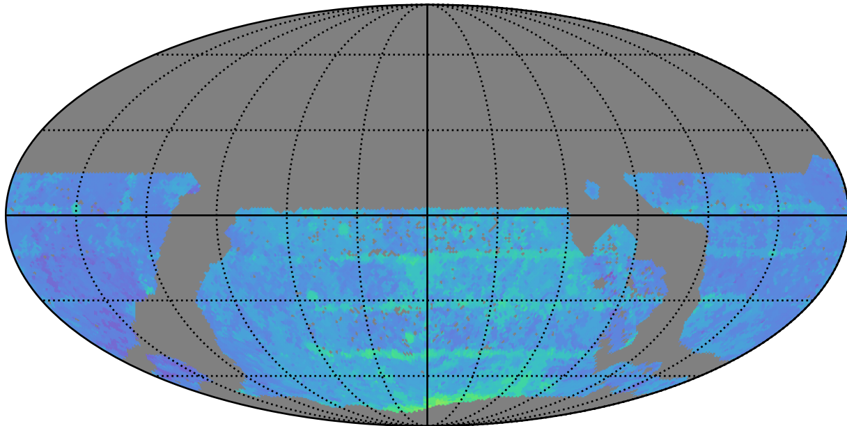
mw_roll_all_v3.3_10yrs WFD y band: 80thPercentile Season Length
