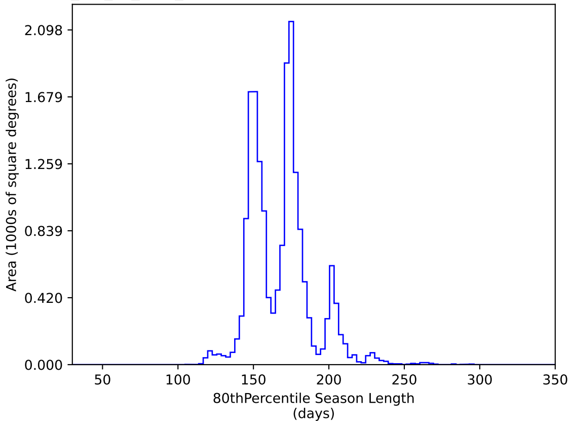
mw_roll_all_v3.3_10yrs WFD y band: 80thPercentile Season Length
