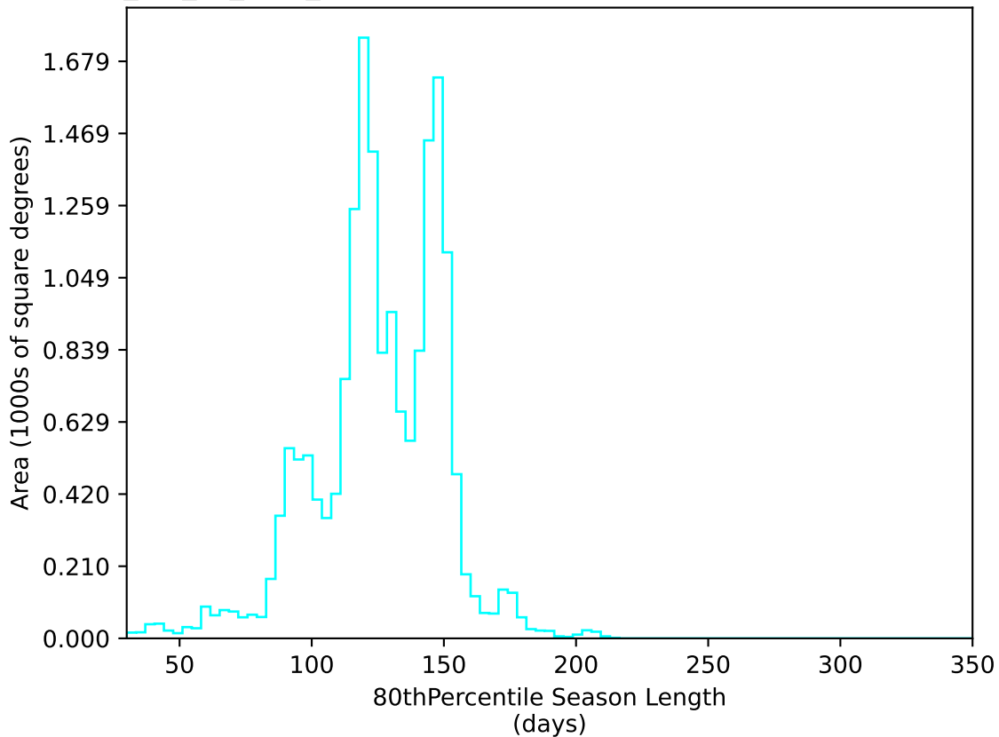
mw_roll_all_v3.3_10yrs WFD u band: 80thPercentile Season Length
