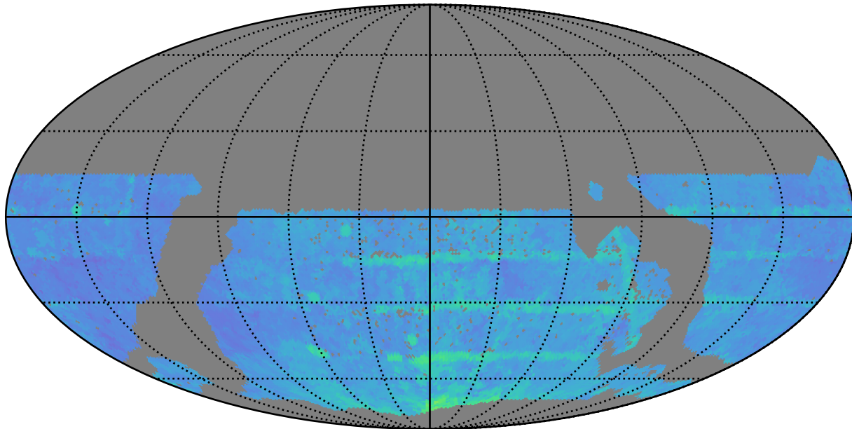
mw_roll_all_v3.3_10yrs WFD r band: 80thPercentile Season Length
