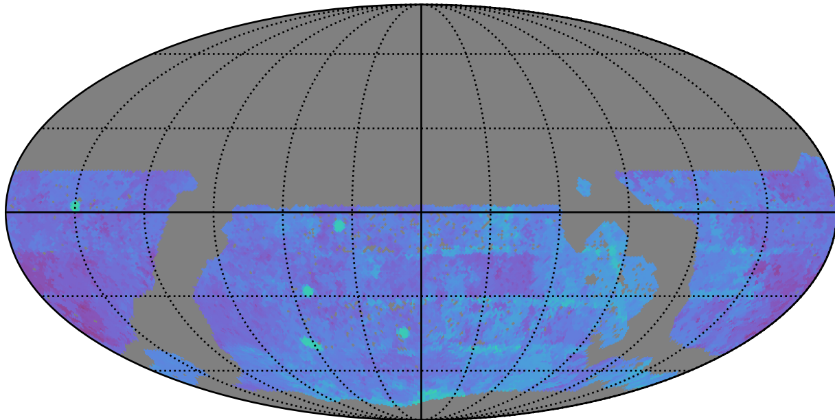
mw_roll_all_v3.3_10yrs WFD g band: 80thPercentile Season Length
