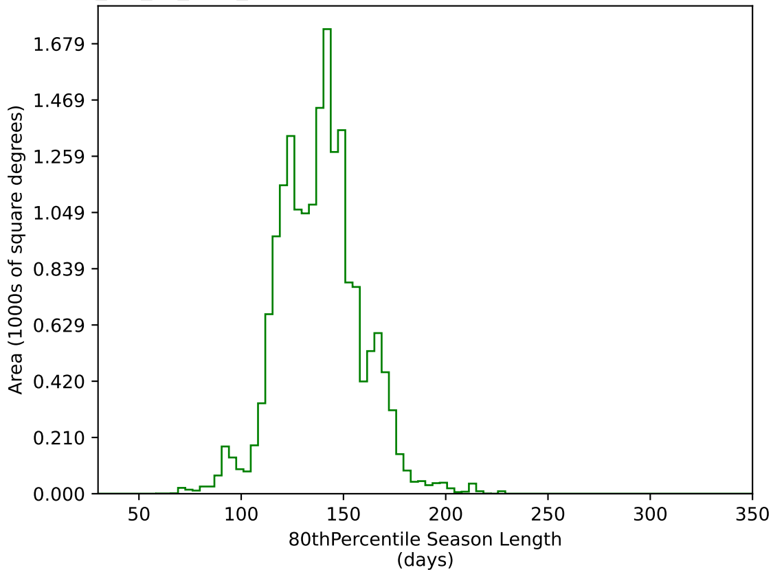
mw_roll_all_v3.3_10yrs WFD g band: 80thPercentile Season Length
