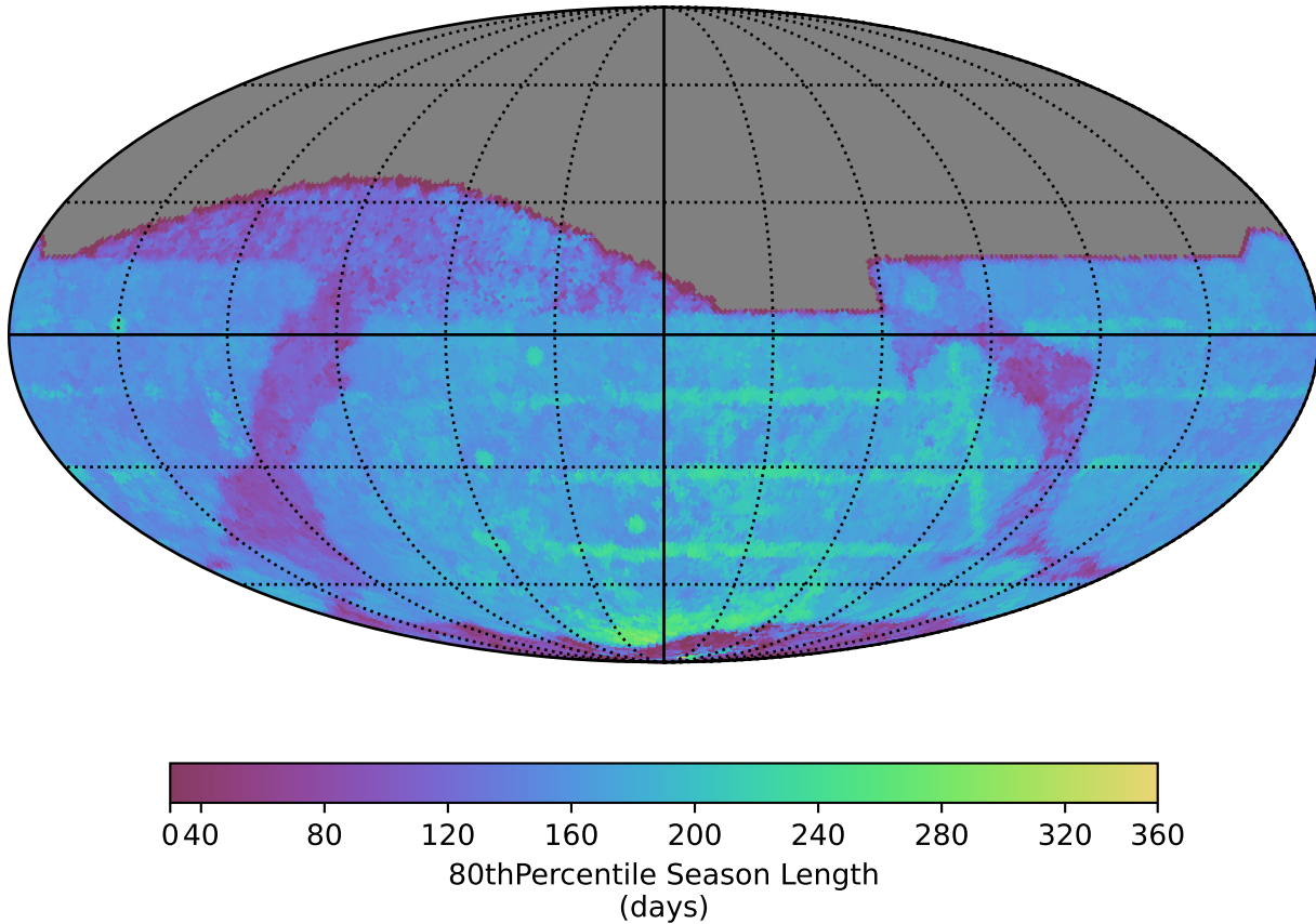
mw_roll_all_v3.3_10yrs All sky z band: 80thPercentile Season Length
