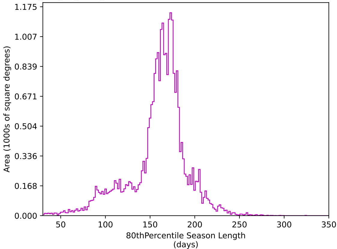
mw_roll_all_v3.3_10yrs All sky z band: 80thPercentile Season Length
