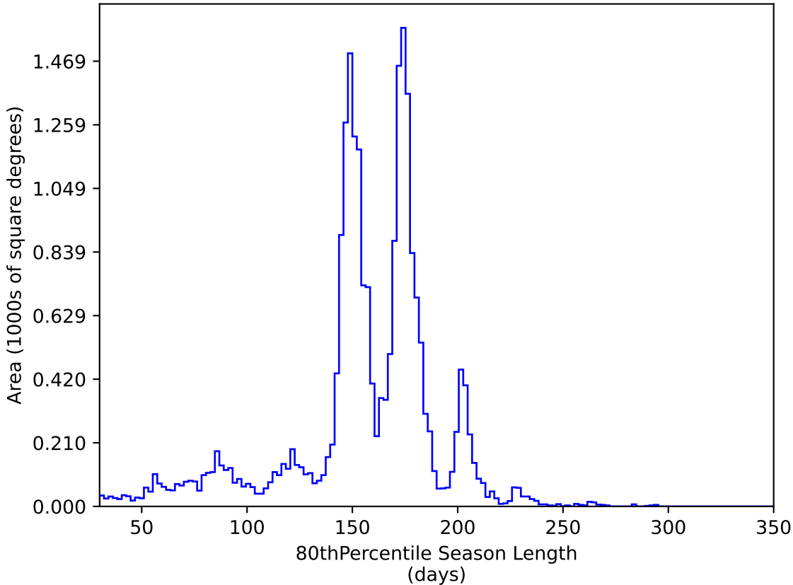
mw_roll_all_v3.3_10yrs All sky y band: 80thPercentile Season Length
