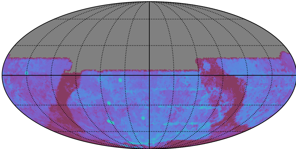
mw_roll_all_v3.3_10yrs All sky u band: 80thPercentile Season Length
