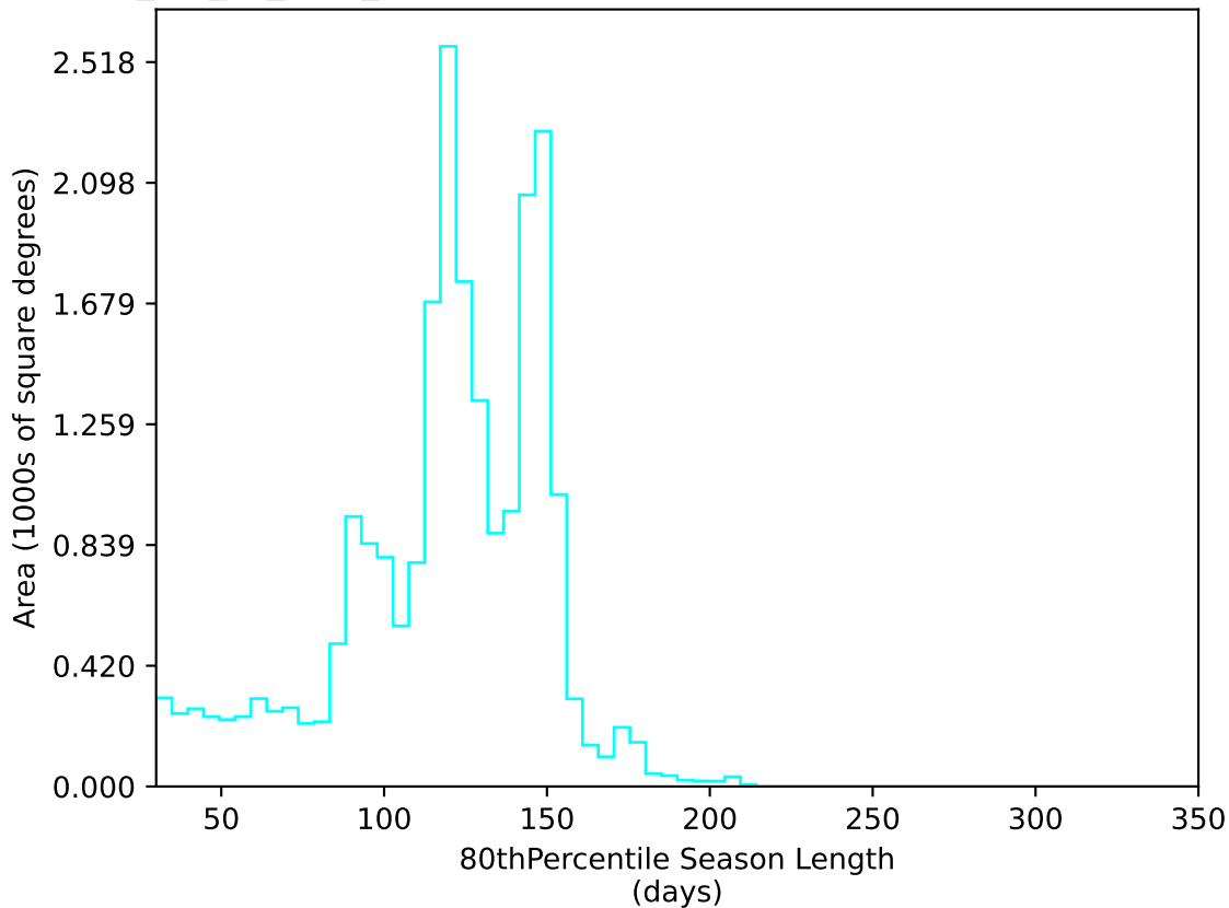
mw_roll_all_v3.3_10yrs All sky u band: 80thPercentile Season Length
