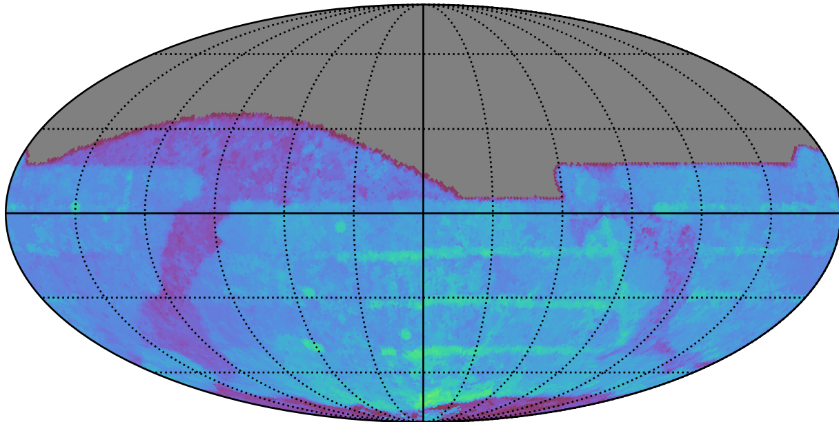
mw_roll_all_v3.3_10yrs All sky r band: 80thPercentile Season Length
