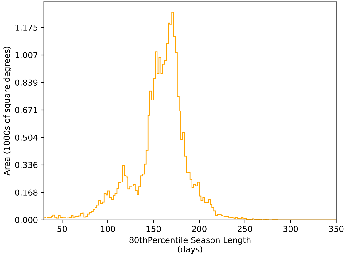
mw_roll_all_v3.3_10yrs All sky r band: 80thPercentile Season Length
