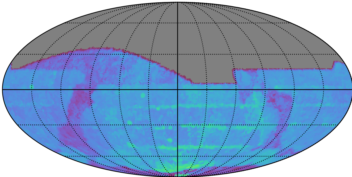
mw_roll_all_v3.3_10yrs All sky i band: 80thPercentile Season Length
