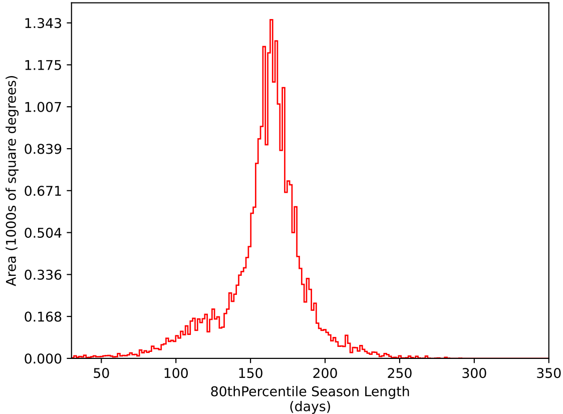
mw_roll_all_v3.3_10yrs All sky i band: 80thPercentile Season Length
