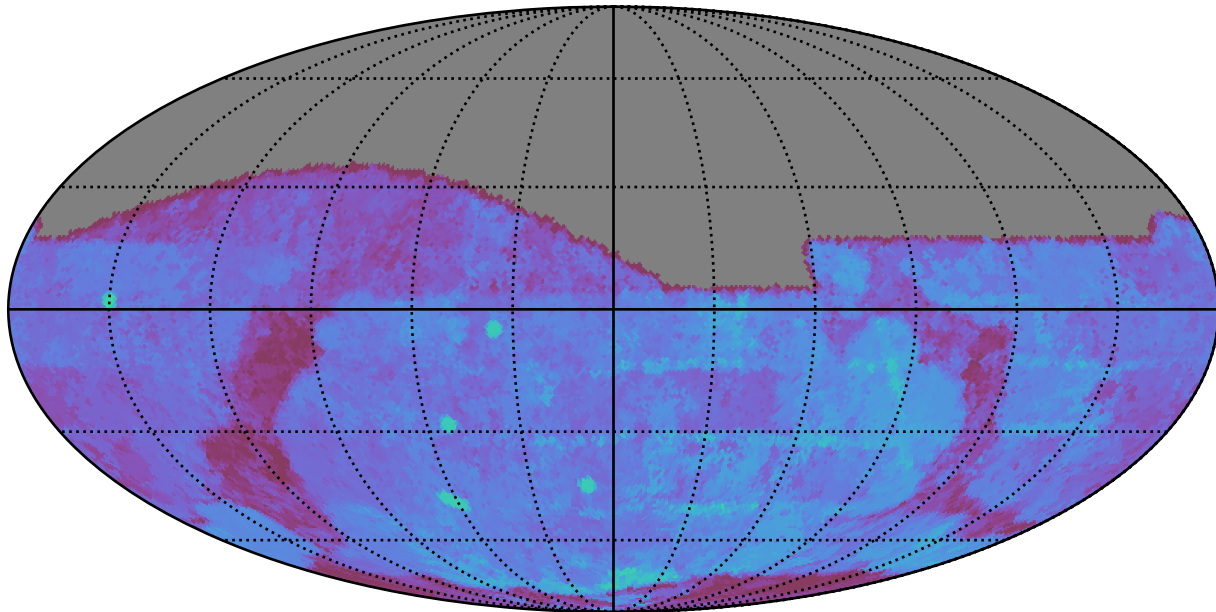
mw_roll_all_v3.3_10yrs All sky g band: 80thPercentile Season Length
