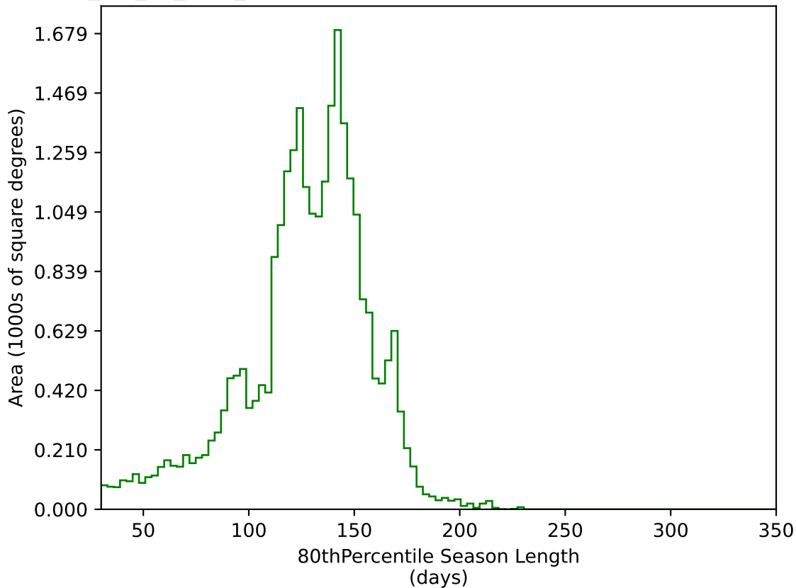
mw_roll_all_v3.3_10yrs All sky g band: 80thPercentile Season Length
