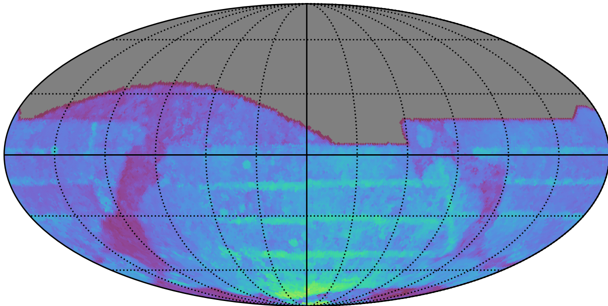
mw_roll_all_v3.3_10yrs All sky all bands: 80thPercentile Season Length
