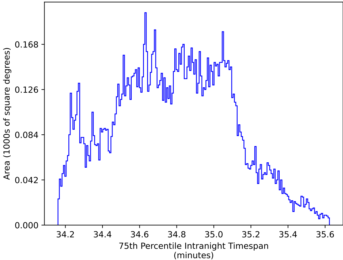
mw_roll_all_v3.3_10yrs WFD zy bands: 75th Percentile Intranight Timespan
