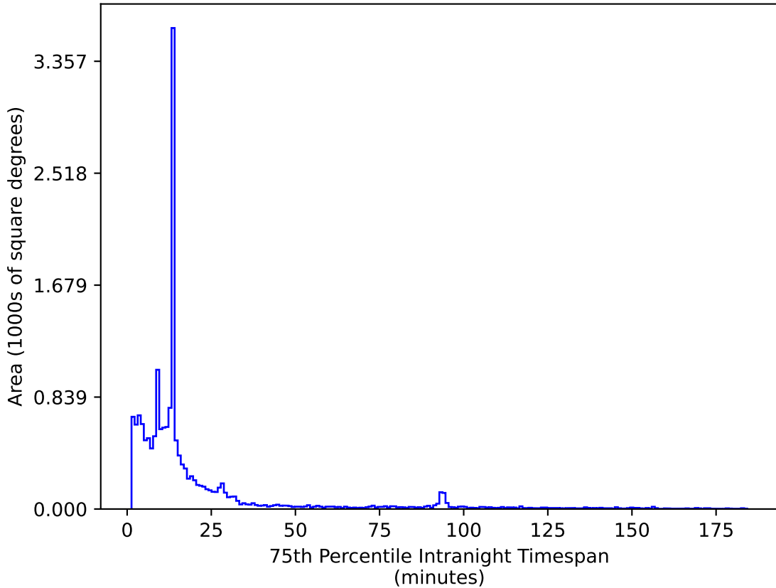
mw_roll_all_v3.3_10yrs WFD z band: 75th Percentile Intranight Timespan
