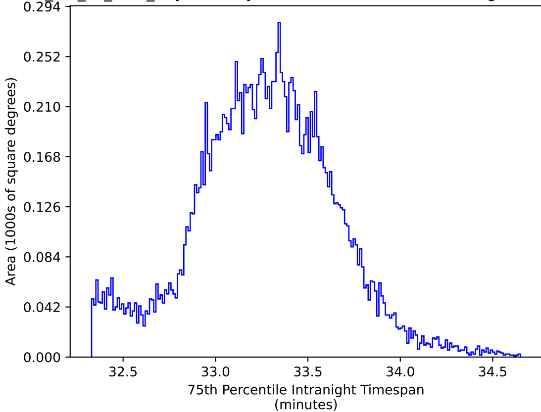
mw_roll_all_v3.3_10yrs WFD y band: 75th Percentile Intranight Timespan
