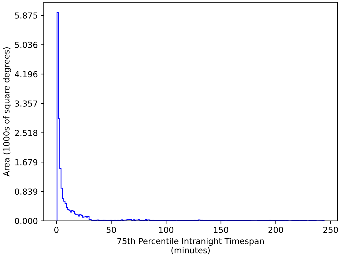
mw_roll_all_v3.3_10yrs WFD u band: 75th Percentile Intranight Timespan
