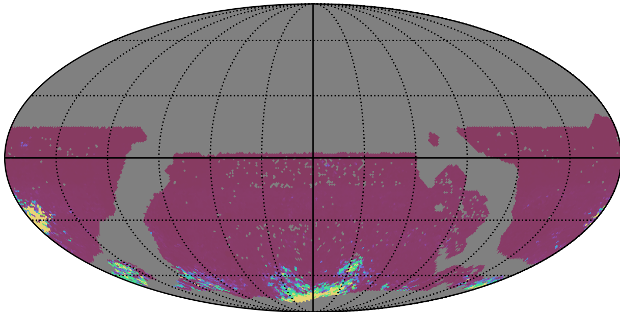
mw_roll_all_v3.3_10yrs WFD ri bands: 75th Percentile Intranight Timespan
