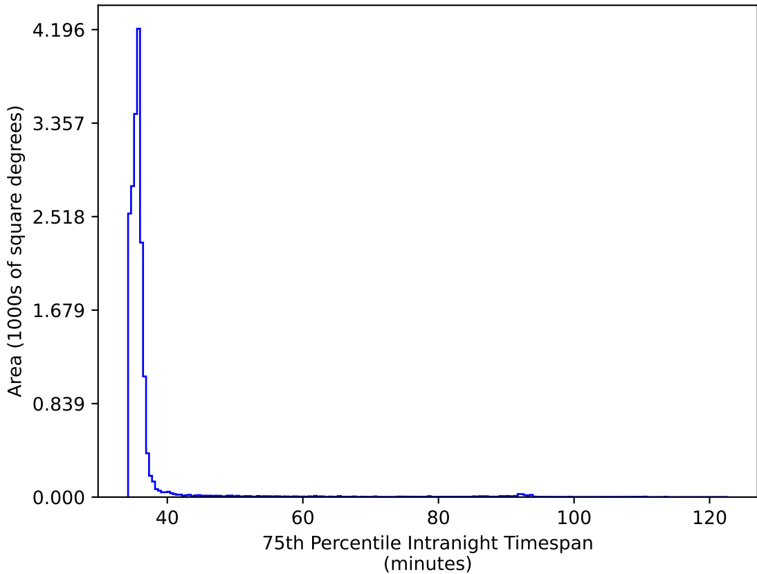
mw_roll_all_v3.3_10yrs WFD ri bands: 75th Percentile Intranight Timespan
