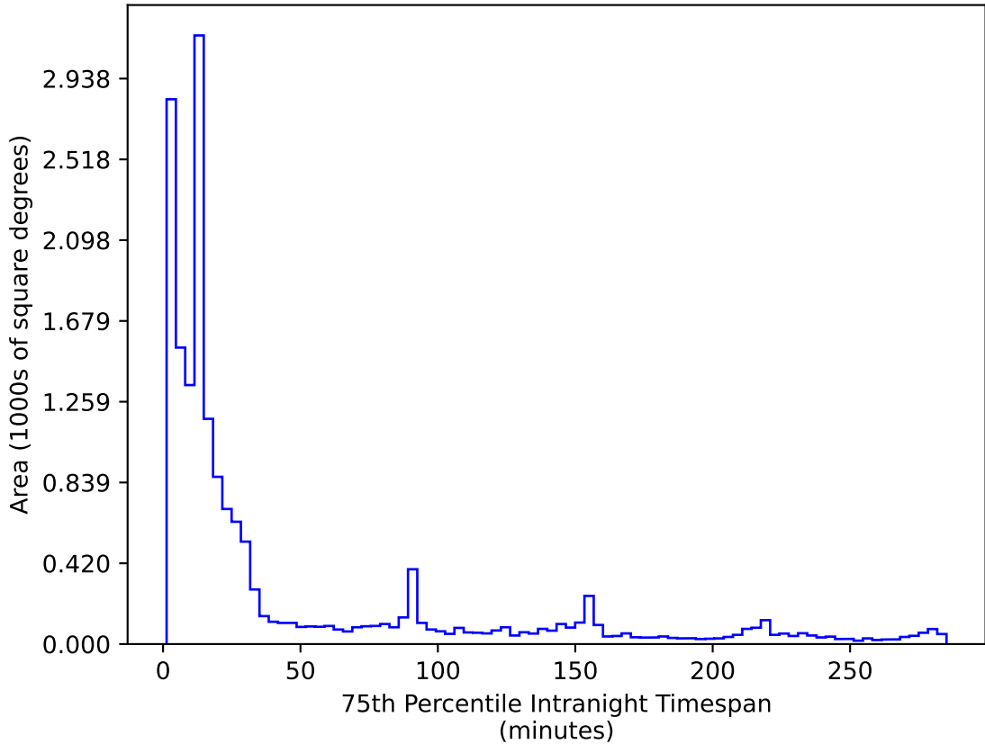
mw_roll_all_v3.3_10yrs WFD r band: 75th Percentile Intranight Timespan
