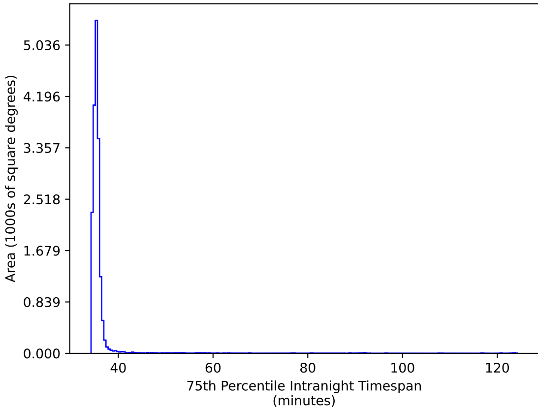
mw_roll_all_v3.3_10yrs WFD gr bands: 75th Percentile Intranight Timespan
