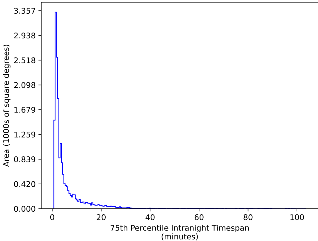
mw_roll_all_v3.3_10yrs WFD g band: 75th Percentile Intranight Timespan
