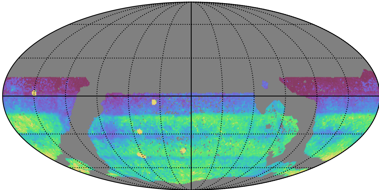
mw_roll_all_v3.3_10yrs WFD: 75th Percentile Intranight Timespan
