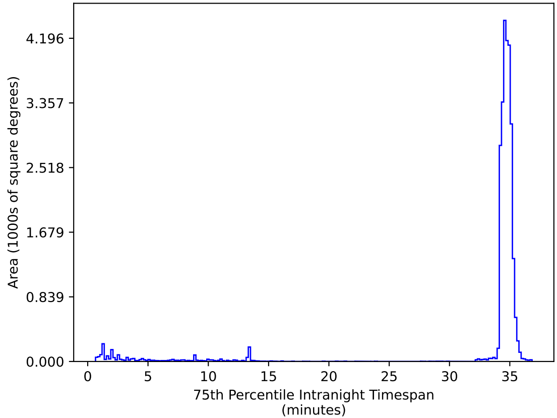
mw_roll_all_v3.3_10yrs All sky zy bands: 75th Percentile Intranight Timespan
