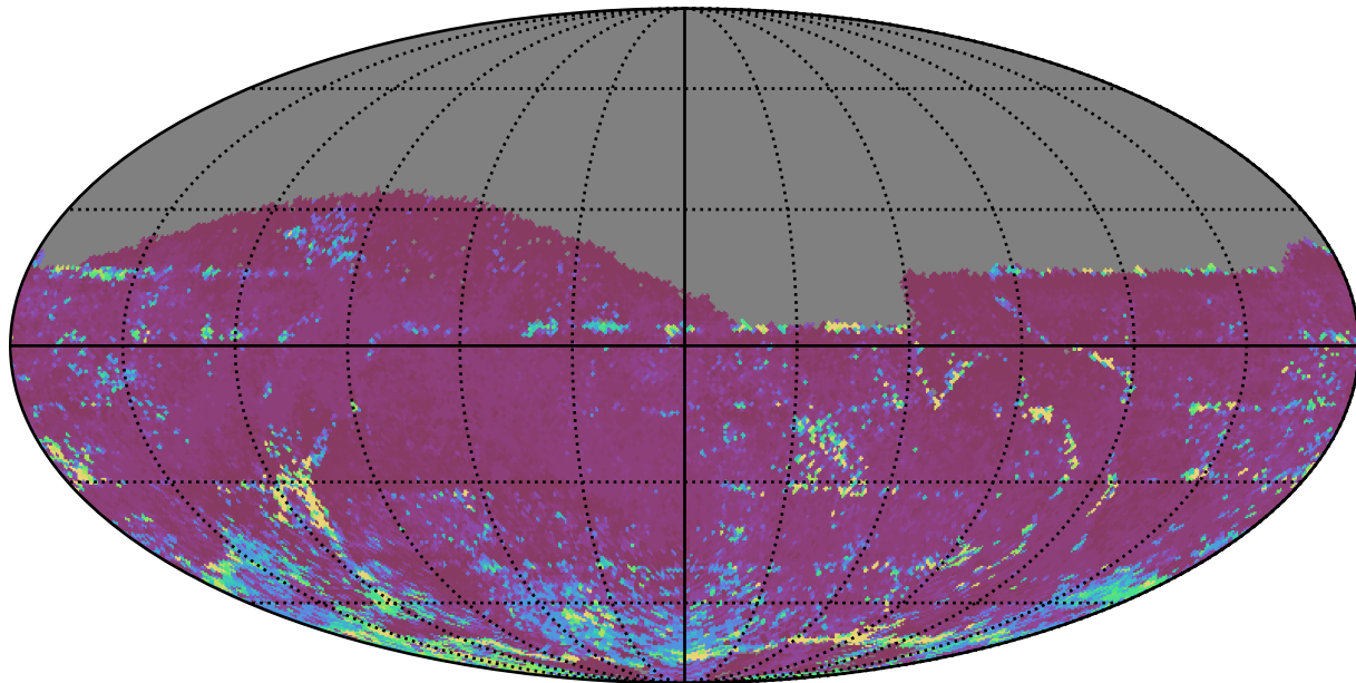
mw_roll_all_v3.3_10yrs All sky z band: 75th Percentile Intranight Timespan
