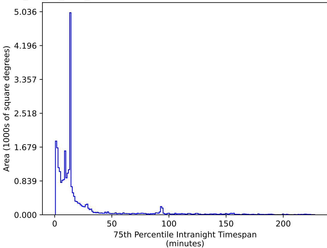
mw_roll_all_v3.3_10yrs All sky z band: 75th Percentile Intranight Timespan
