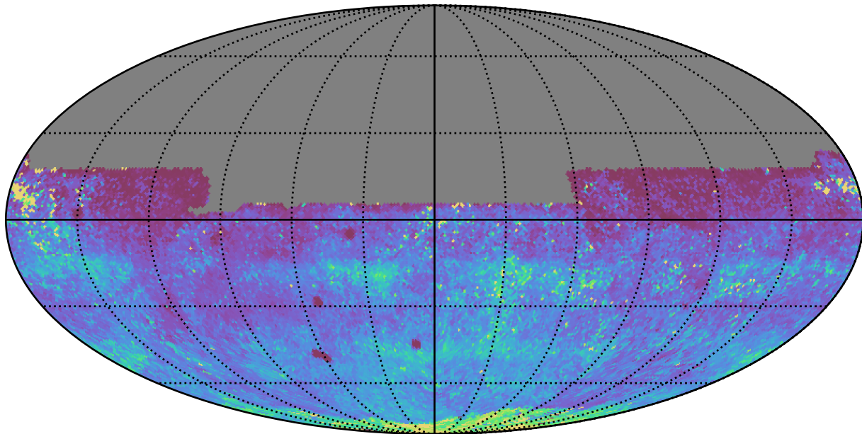
mw_roll_all_v3.3_10yrs All sky y band: 75th Percentile Intranight Timespan
