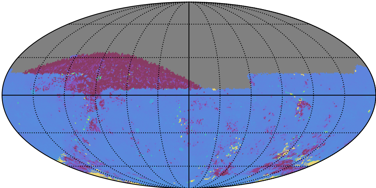
mw_roll_all_v3.3_10yrs All sky ug bands: 75th Percentile Intranight Timespan
