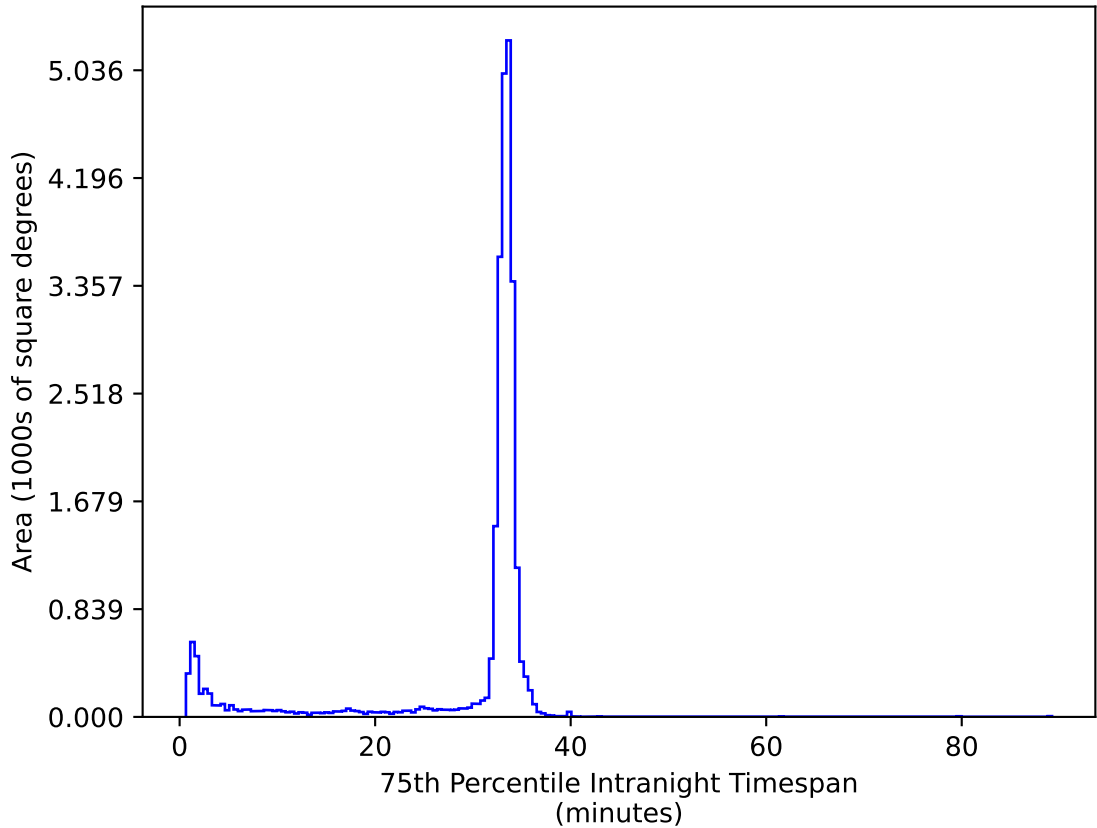
mw_roll_all_v3.3_10yrs All sky ug bands: 75th Percentile Intranight Timespan
