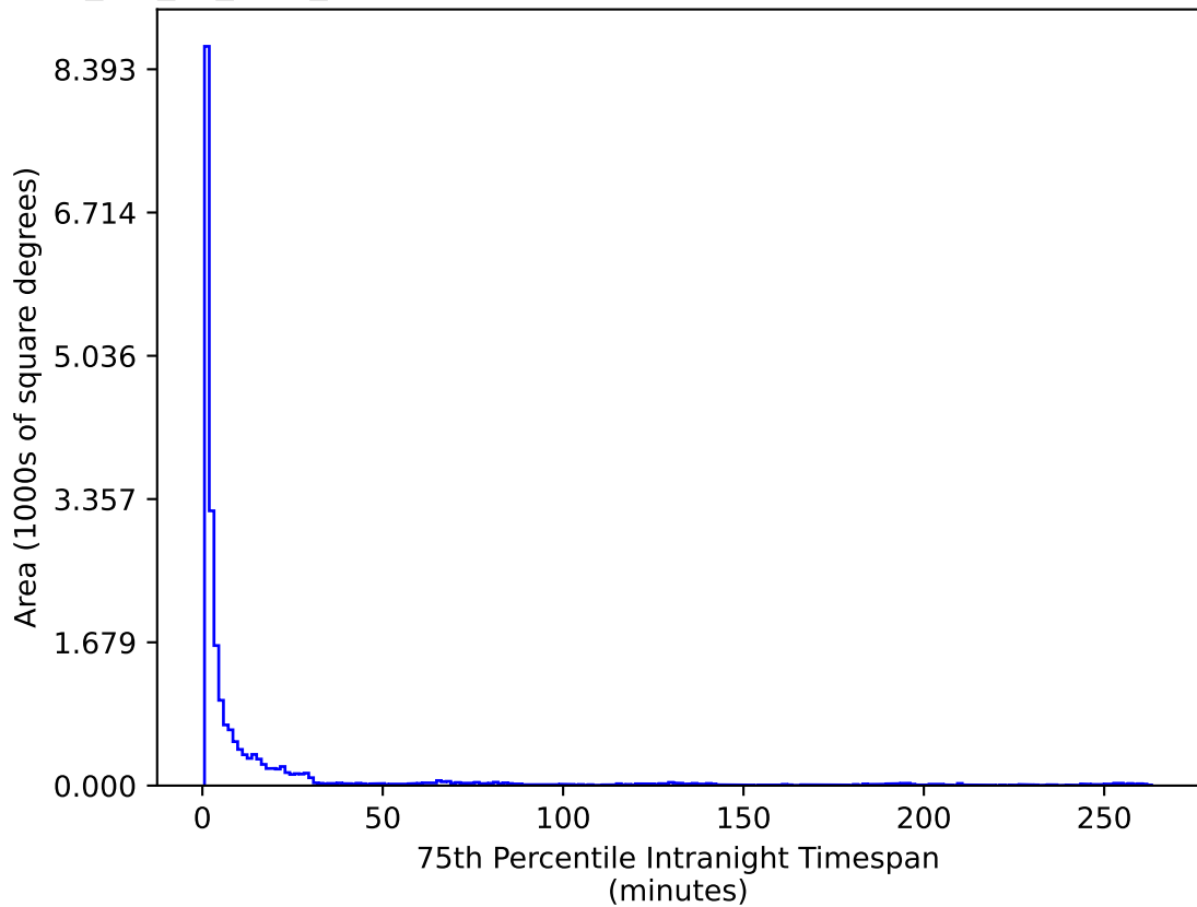
mw_roll_all_v3.3_10yrs All sky u band: 75th Percentile Intranight Timespan
