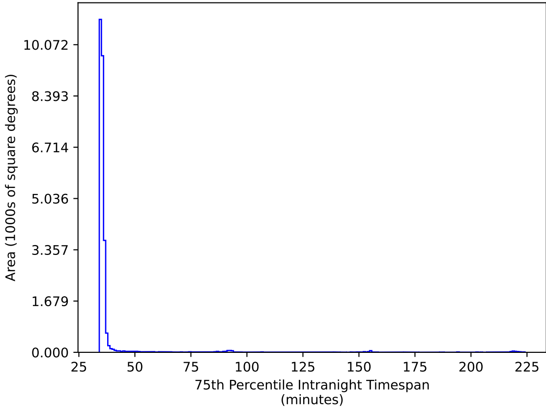
mw_roll_all_v3.3_10yrs All sky ri bands: 75th Percentile Intranight Timespan
