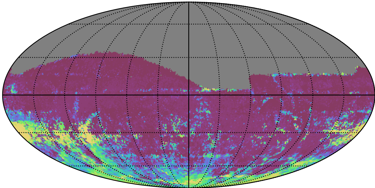
mw_roll_all_v3.3_10yrs All sky r band: 75th Percentile Intranight Timespan
