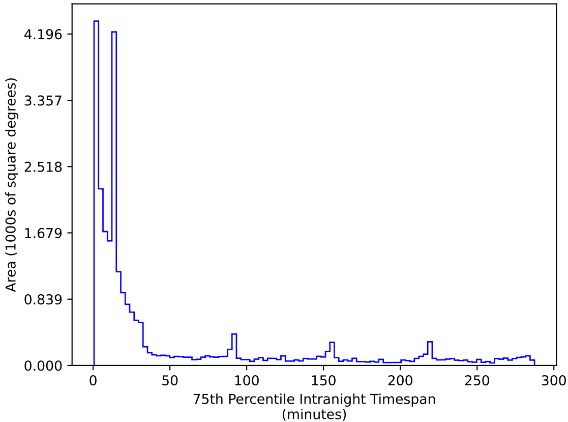
mw_roll_all_v3.3_10yrs All sky r band: 75th Percentile Intranight Timespan
